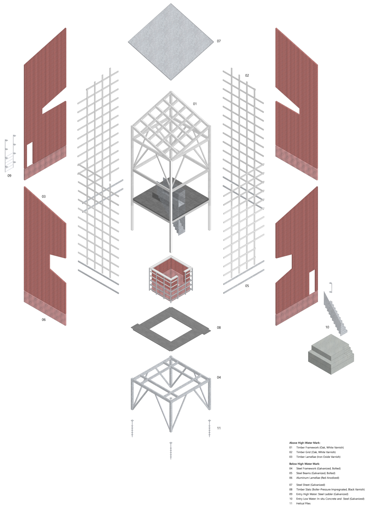
Construction principle.
