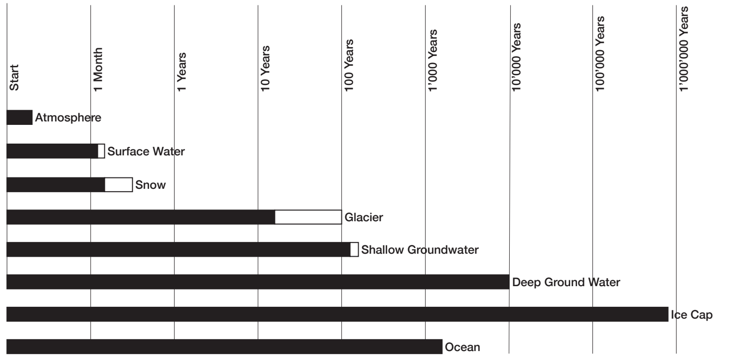
Logarithmic timescale of water in its global circulation.
