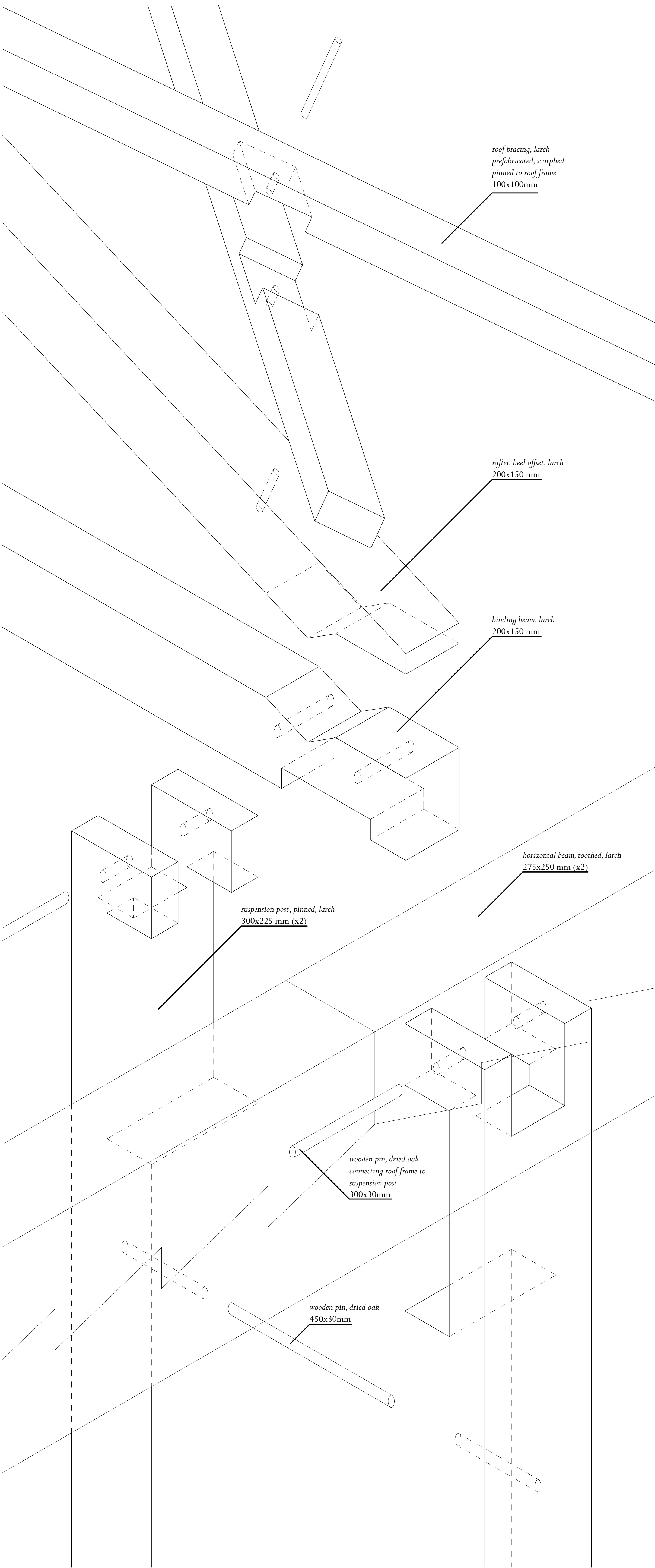
axonometric drawing 1:5
